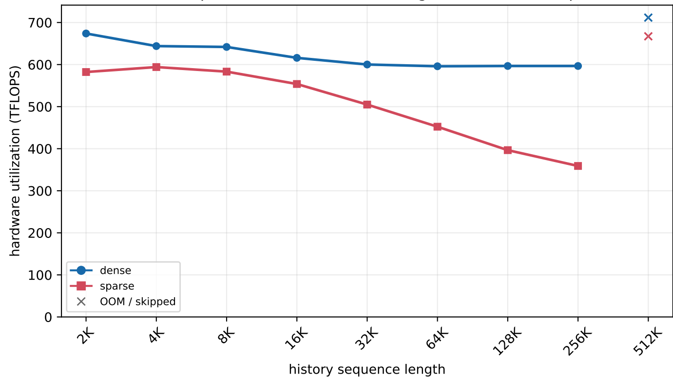
H800 MLA prefill - batch=128, new length=512 (chunked prefill)
