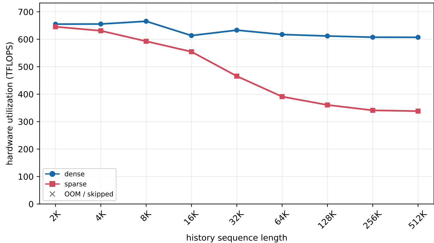
H800 MLA prefill - batch=128, new length=64 (chunked prefill)
