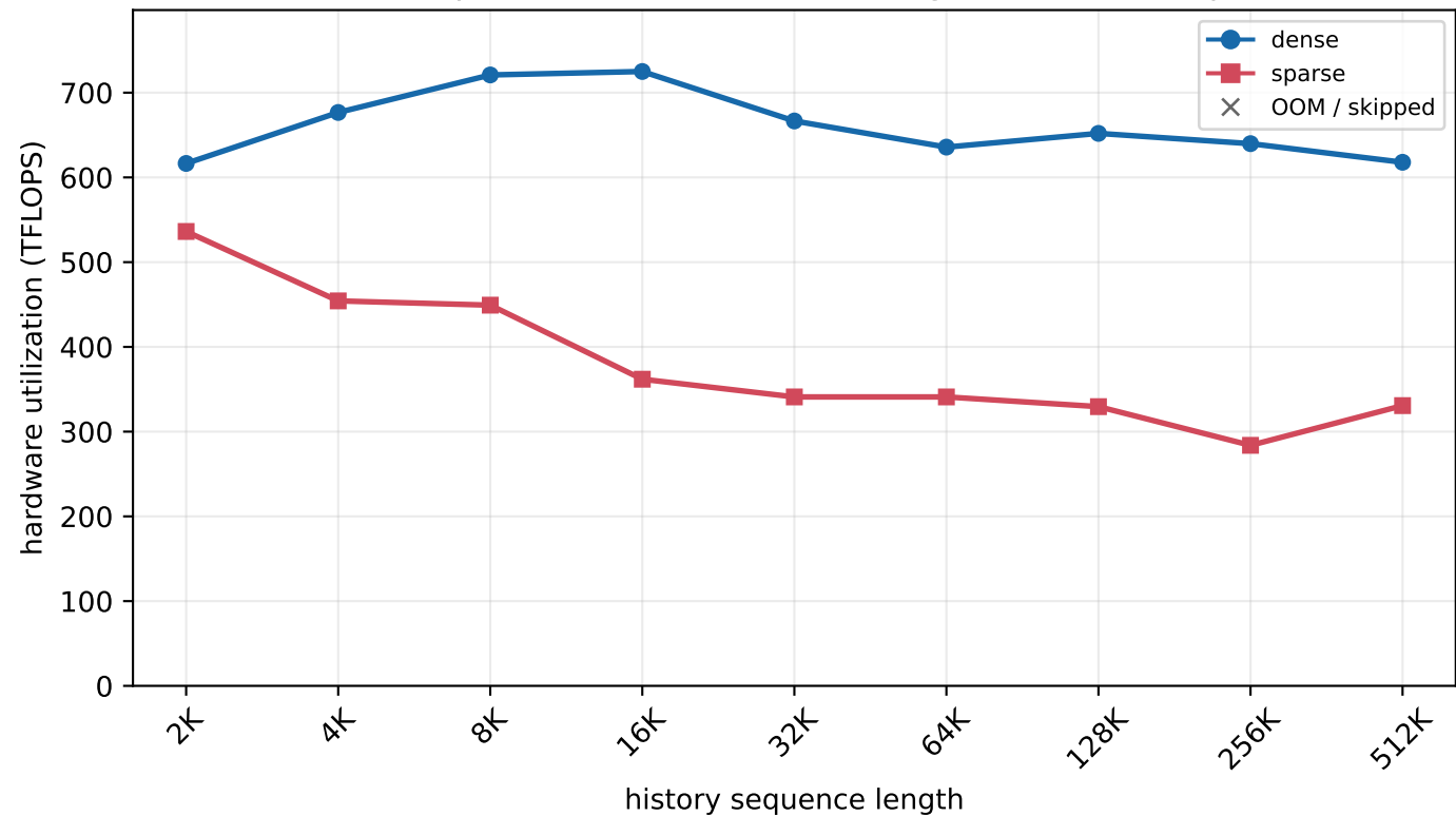
H800 MLA prefill - batch=128, new length=8 (chunked prefill)
