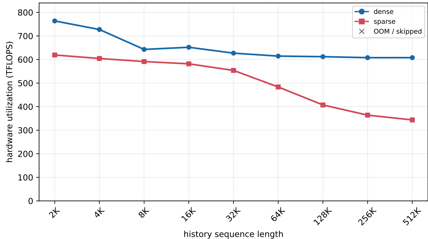
H800 MLA prefill - batch=16, new length=1K (chunked prefill)
