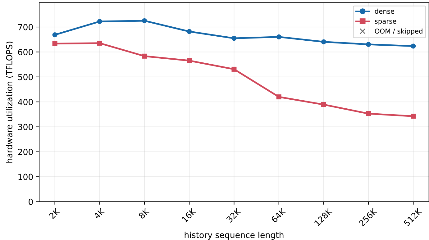
H800 MLA prefill - batch=16, new length=128 (chunked prefill)
