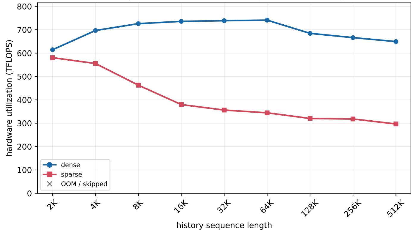
H800 MLA prefill - batch=16, new length=16 (chunked prefill)
