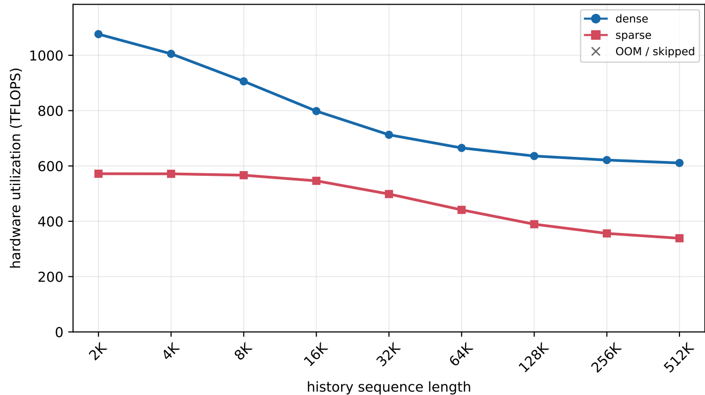
H800 MLA prefill - batch=16, new length=16K (chunked prefill)
