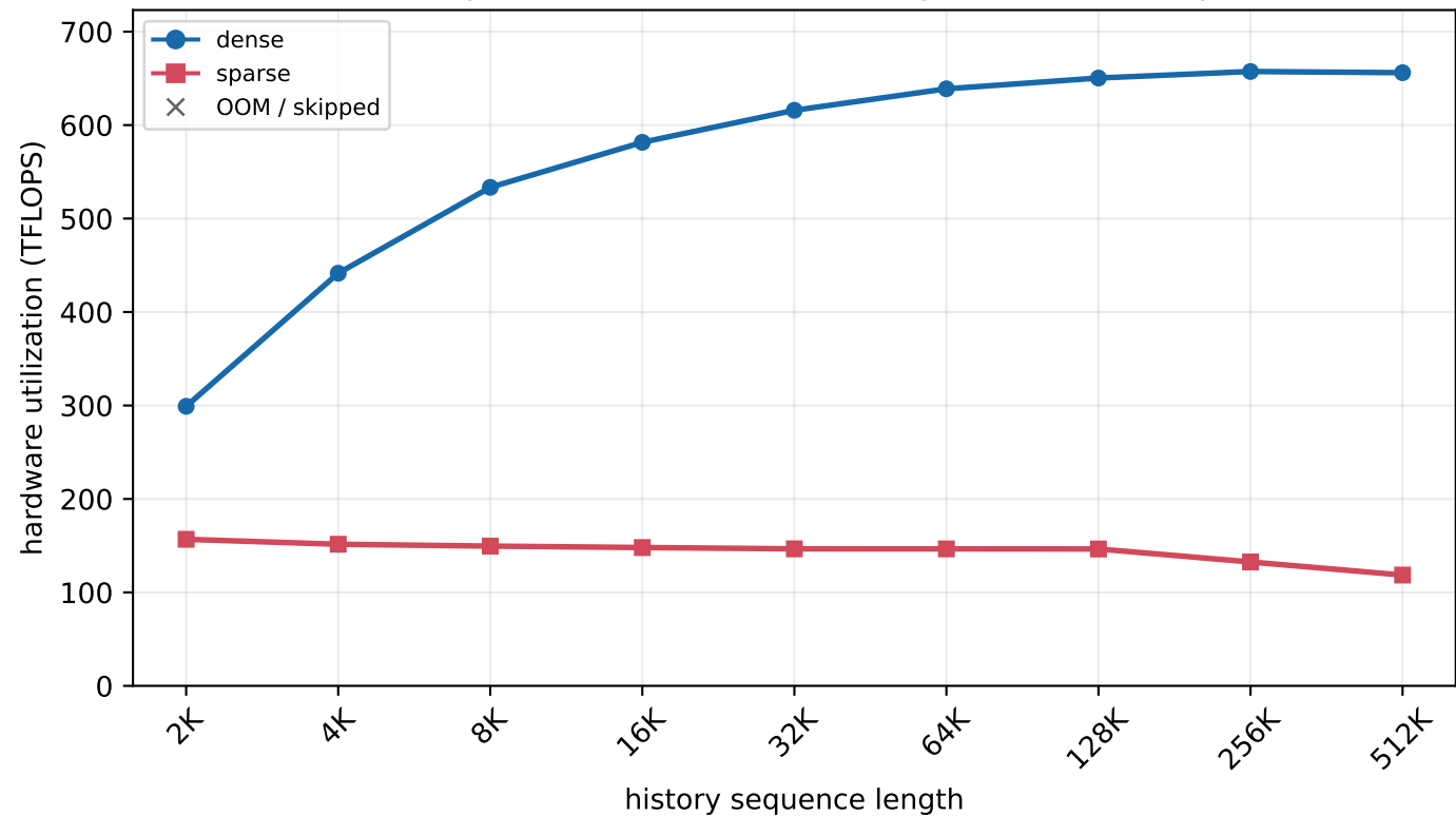
H800 MLA prefill - batch=16, new length=2 (chunked prefill)
