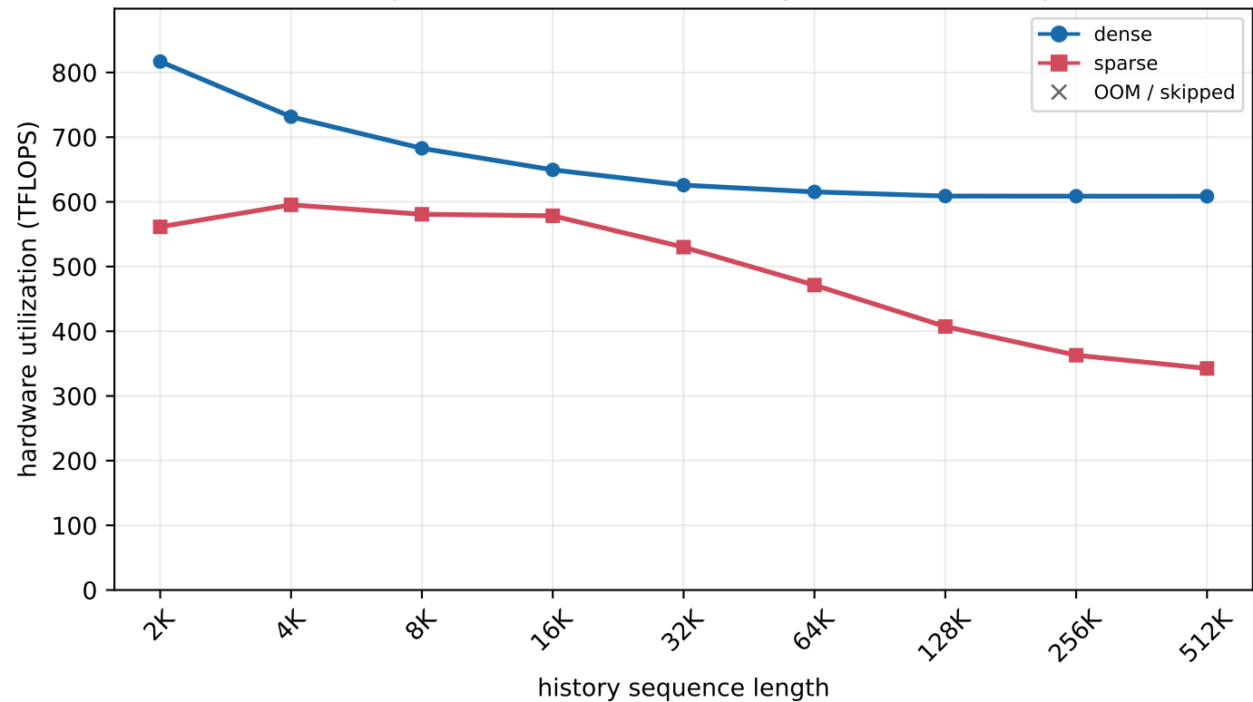
H800 MLA prefill - batch=16, new length=2K (chunked prefill)
