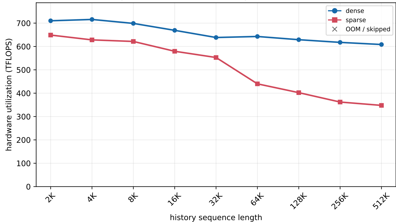
H800 MLA prefill - batch=16, new length=256 (chunked prefill)
