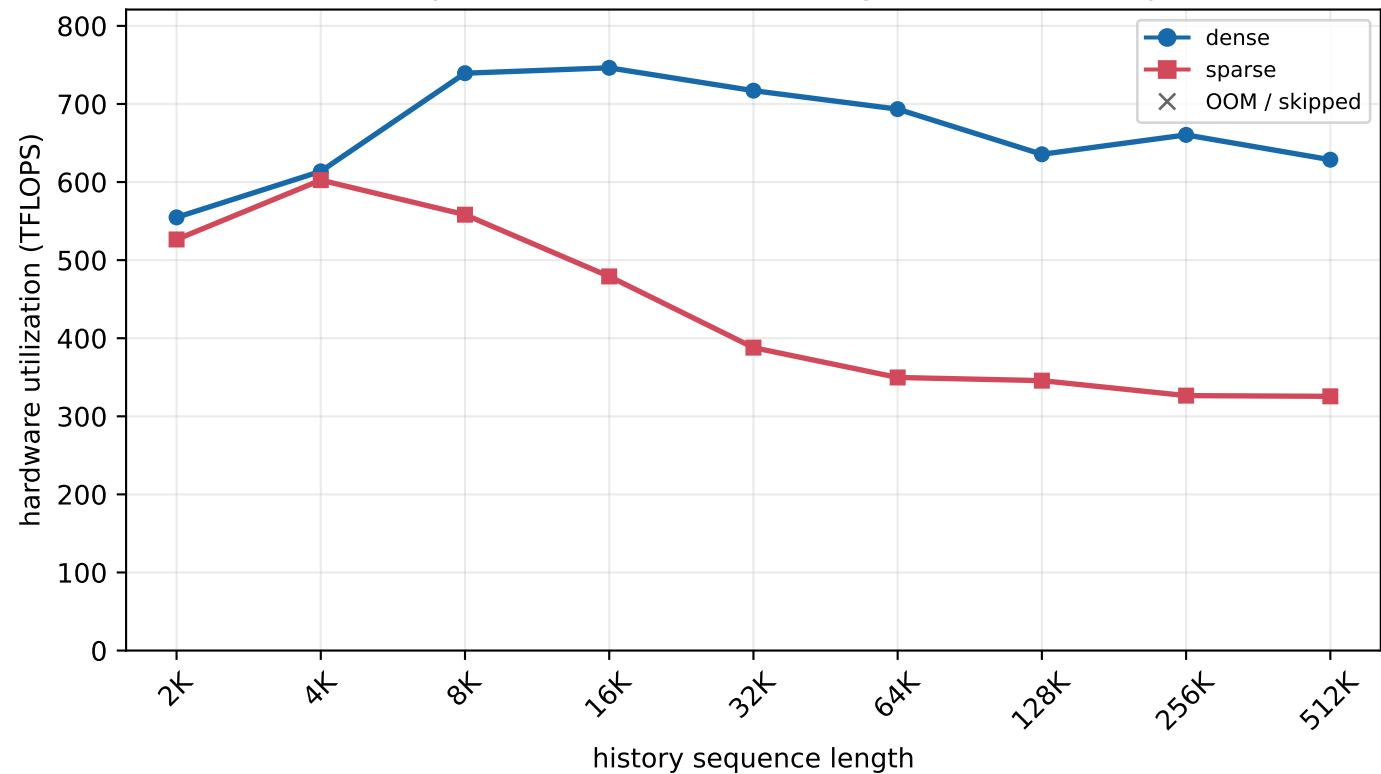
H800 MLA prefill - batch=16, new length=32 (chunked prefill)
