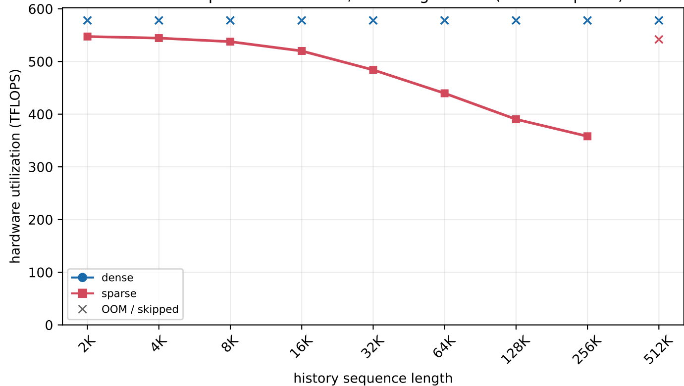
H800 MLA prefill - batch=16, new length=32K (chunked prefill)
