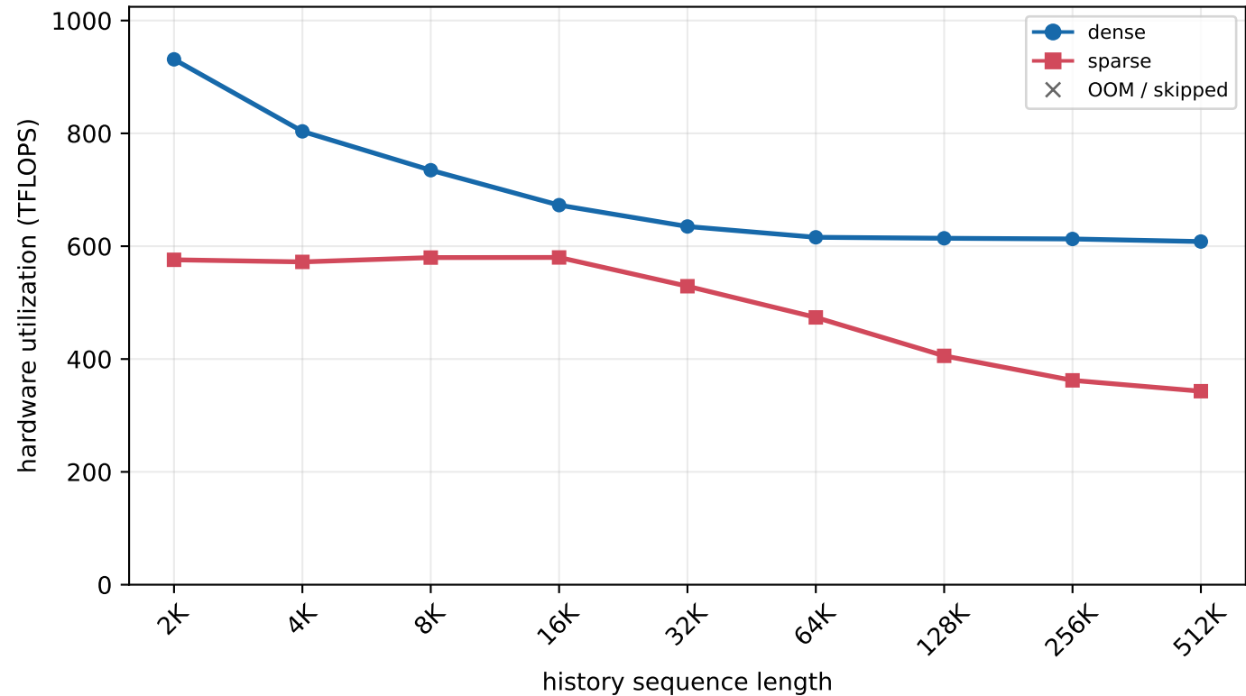
H800 MLA prefill - batch=16, new length=4K (chunked prefill)
