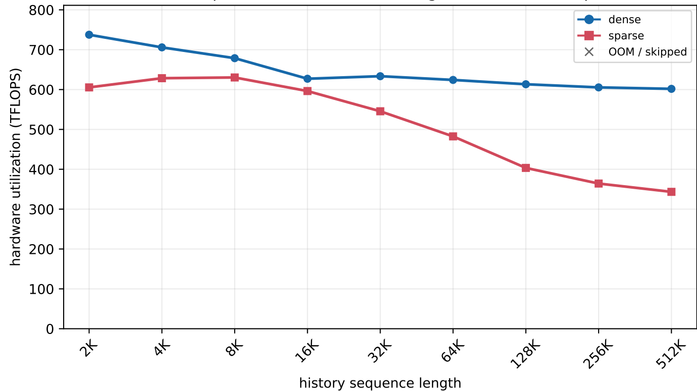
H800 MLA prefill - batch=16, new length=512 (chunked prefill)
