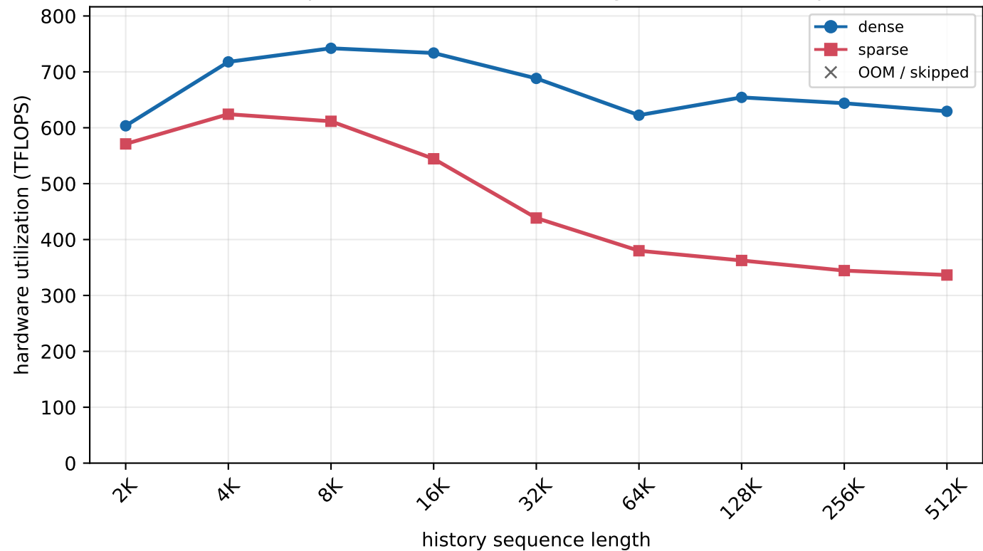
H800 MLA prefill - batch=16, new length=64 (chunked prefill)
