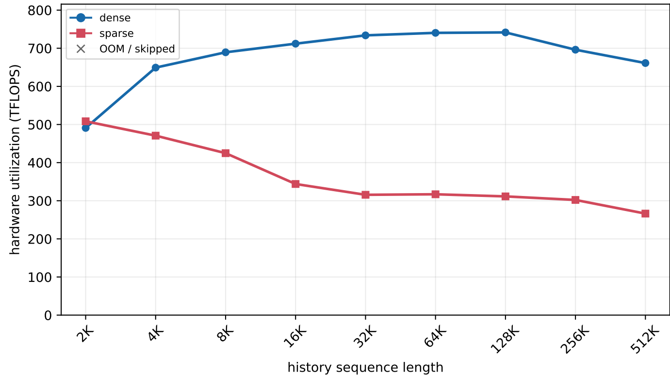
H800 MLA prefill - batch=16, new length=8 (chunked prefill)
