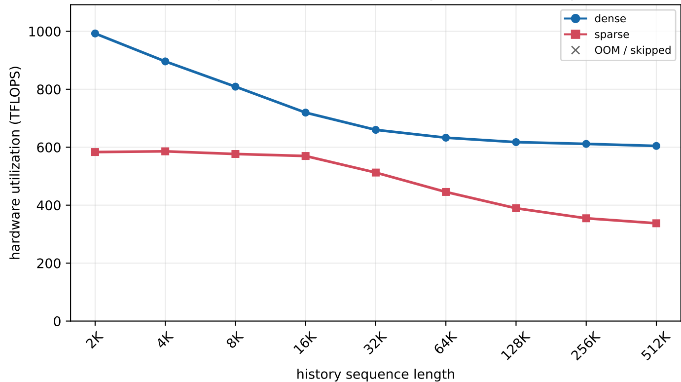
H800 MLA prefill - batch=16, new length=8K (chunked prefill)
