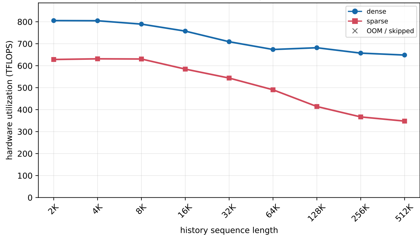
H800 MLA prefill - batch=1, new length=1K (chunked prefill)
