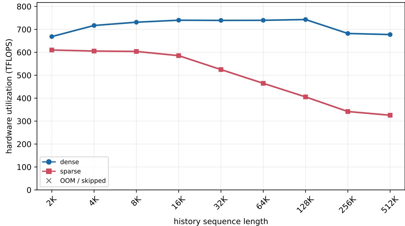
H800 MLA prefill - batch=1, new length=128 (chunked prefill)
