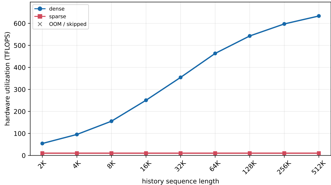
H800 MLA prefill - batch=1, new length=2 (chunked prefill)
