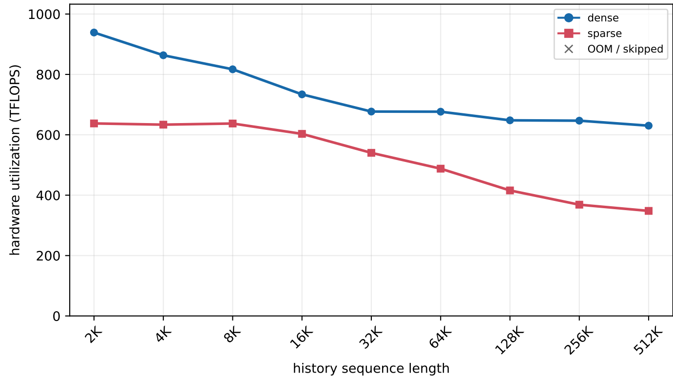
H800 MLA prefill - batch=1, new length=2K (chunked prefill)
