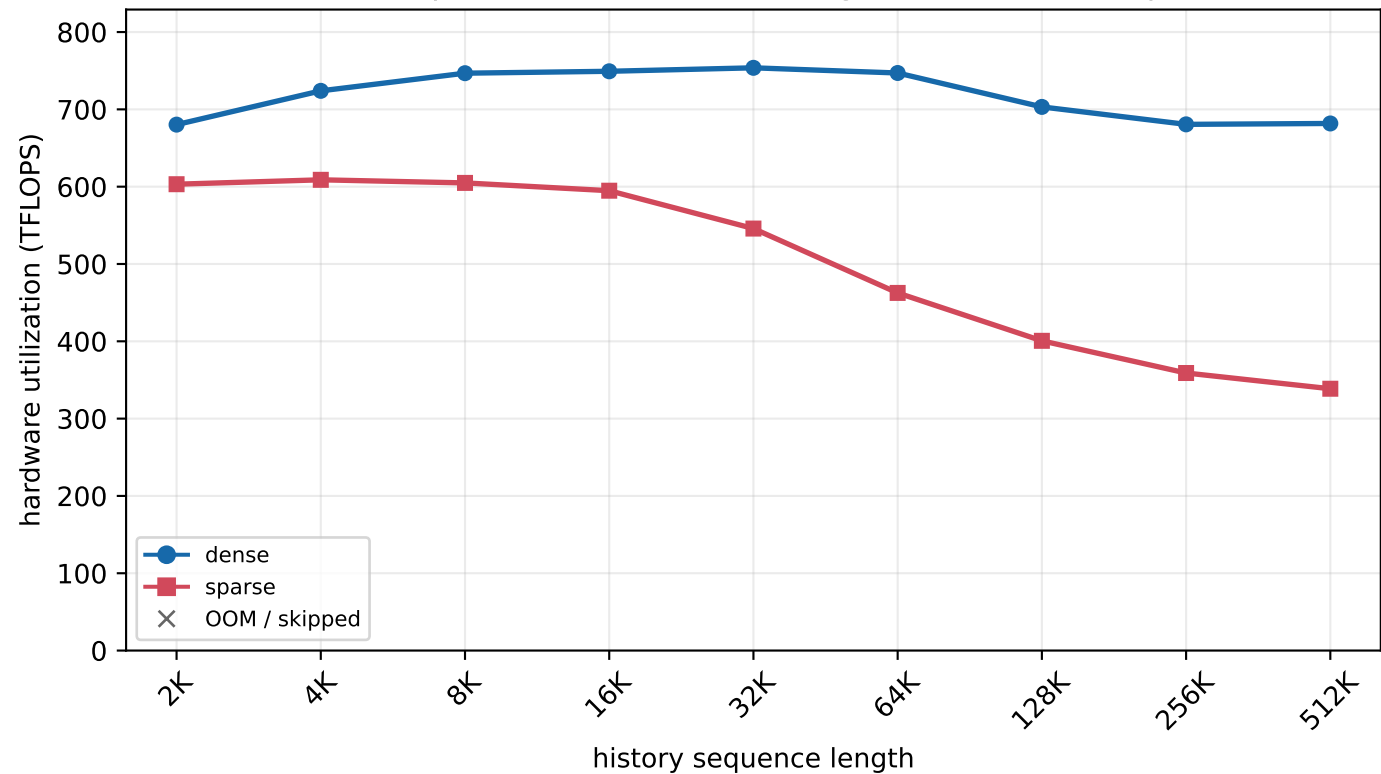
H800 MLA prefill - batch=1, new length=256 (chunked prefill)
