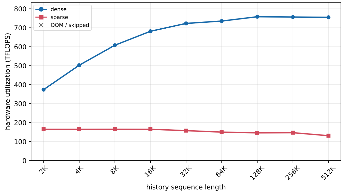
H800 MLA prefill - batch=1, new length=32 (chunked prefill)
