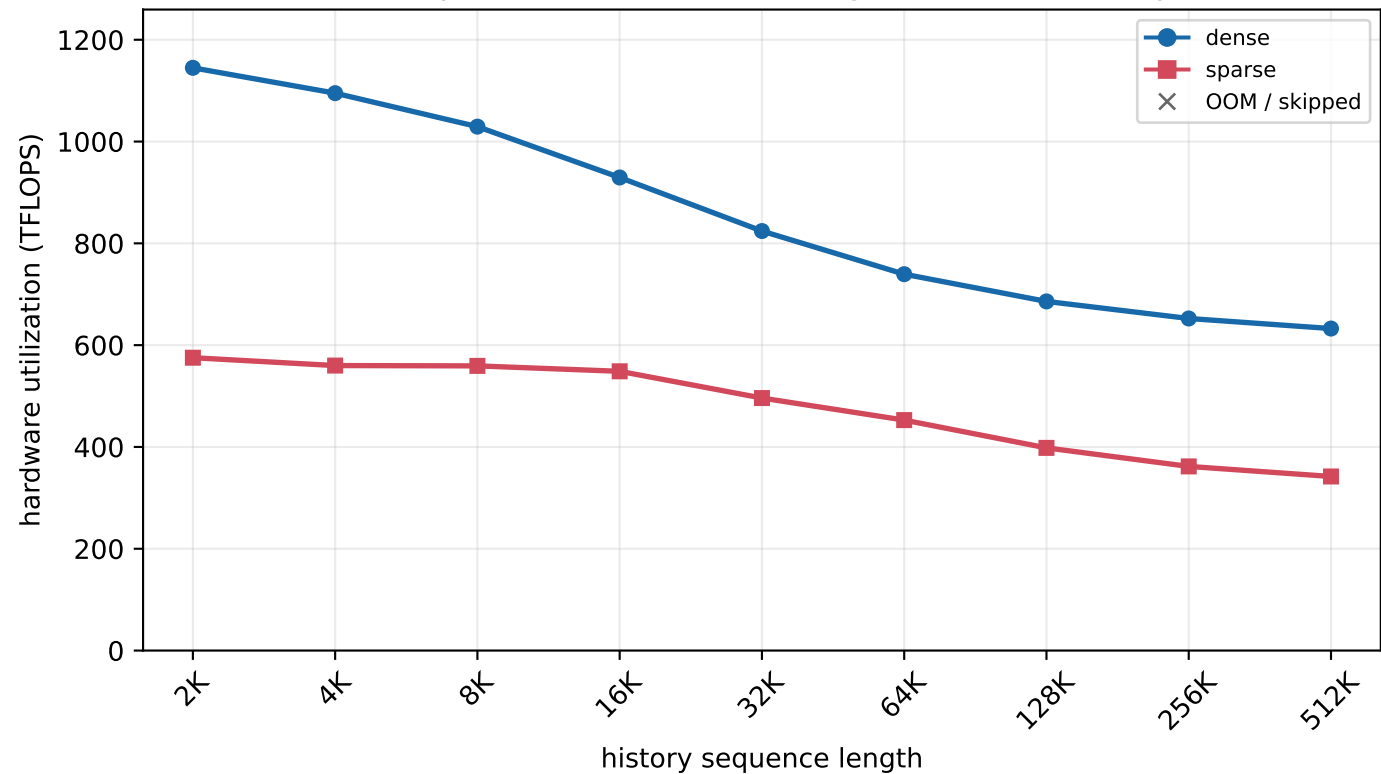
H800 MLA prefill - batch=1, new length=32K (chunked prefill)
