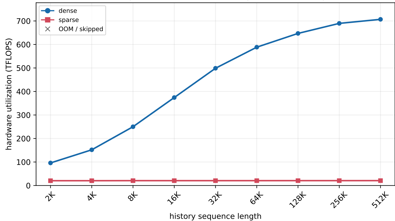
H800 MLA prefill - batch=1, new length=4 (chunked prefill)
