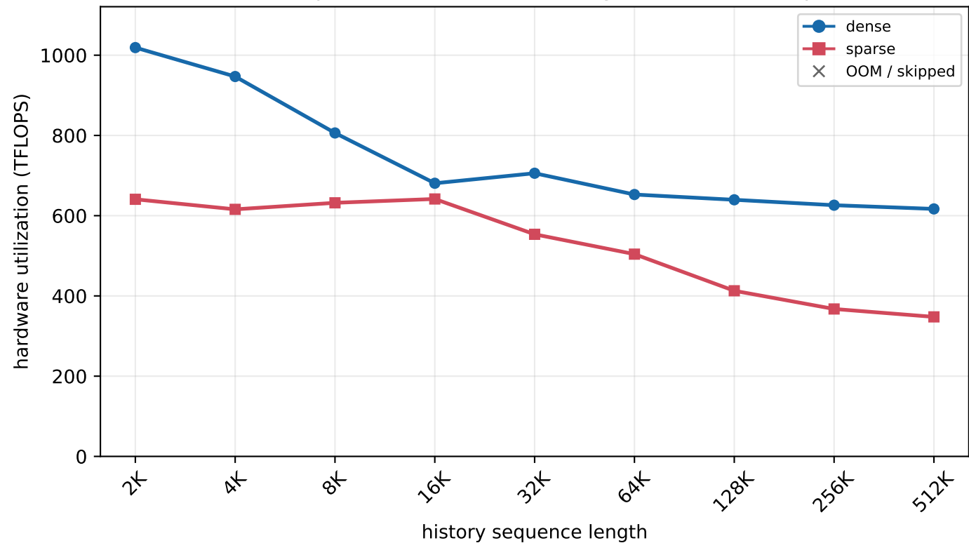
H800 MLA prefill - batch=1, new length=4K (chunked prefill)
