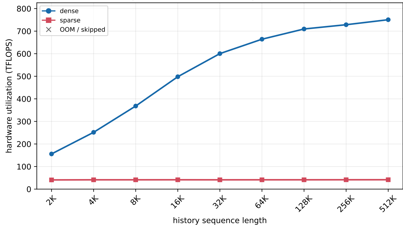
H800 MLA prefill - batch=1, new length=8 (chunked prefill)
