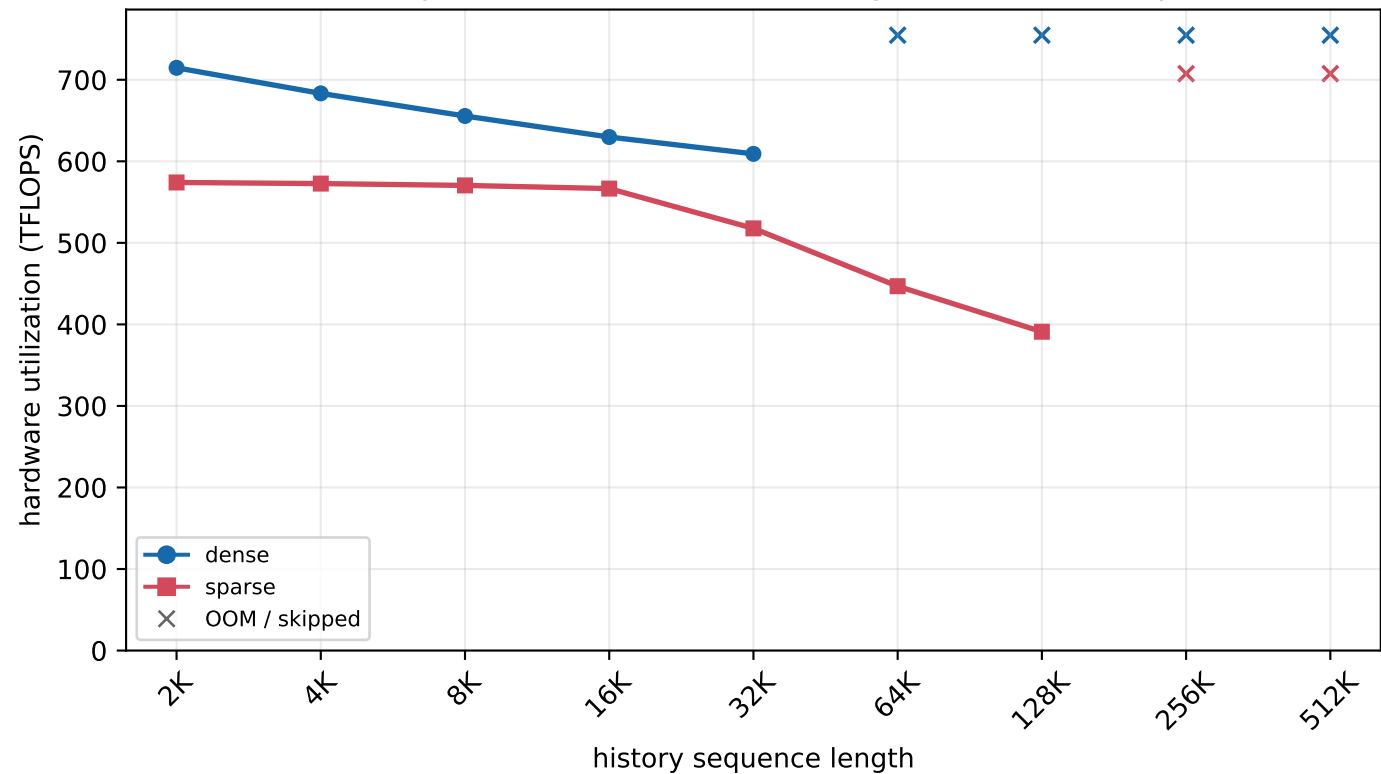
H800 MLA prefill - batch=256, new length=1K (chunked prefill)
