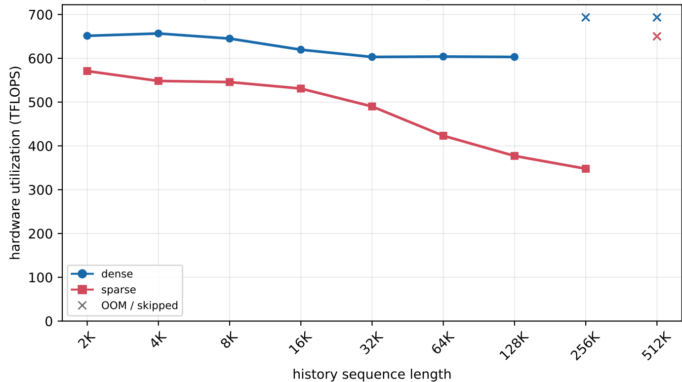
H800 MLA prefill - batch=256, new length=128 (chunked prefill)
