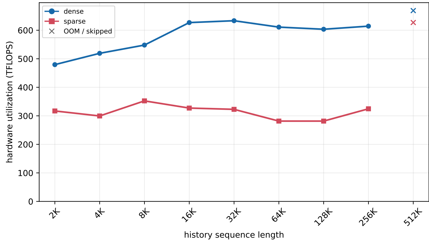
H800 MLA prefill - batch=256, new length=2 (chunked prefill)
