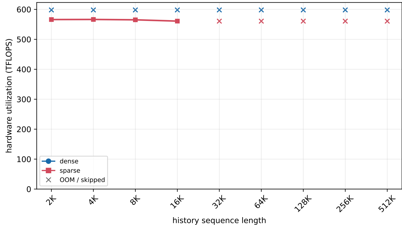
H800 MLA prefill - batch=256, new length=2K (chunked prefill)
