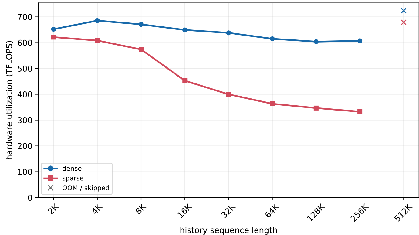
H800 MLA prefill - batch=256, new length=32 (chunked prefill)
