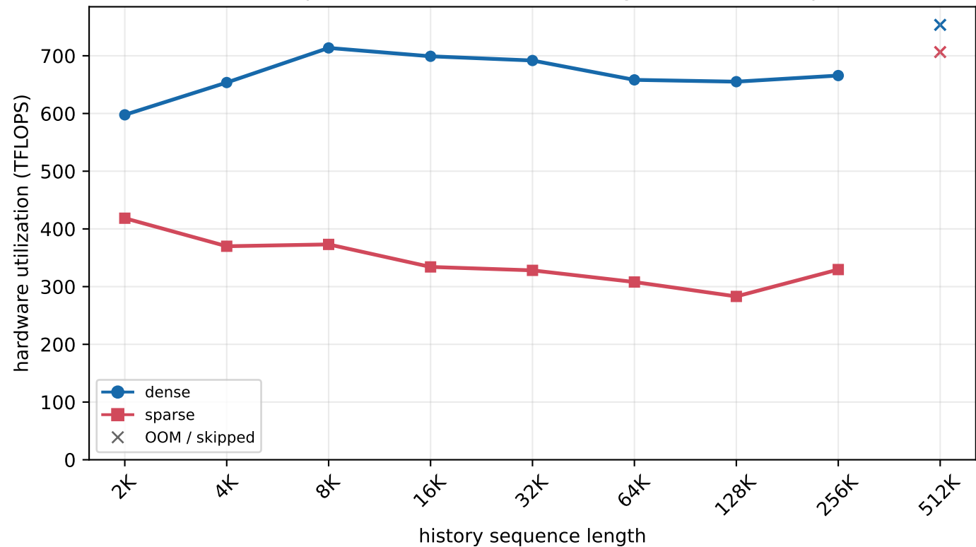
H800 MLA prefill - batch=256, new length=4 (chunked prefill)
