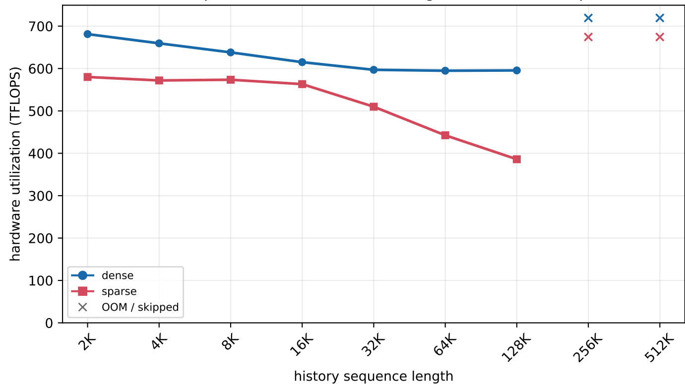
H800 MLA prefill - batch=256, new length=512 (chunked prefill)
