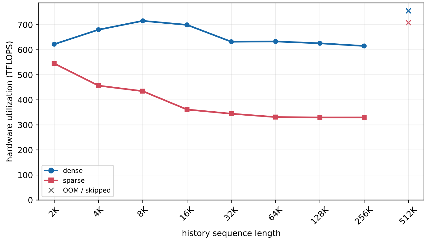
H800 MLA prefill - batch=256, new length=8 (chunked prefill)
