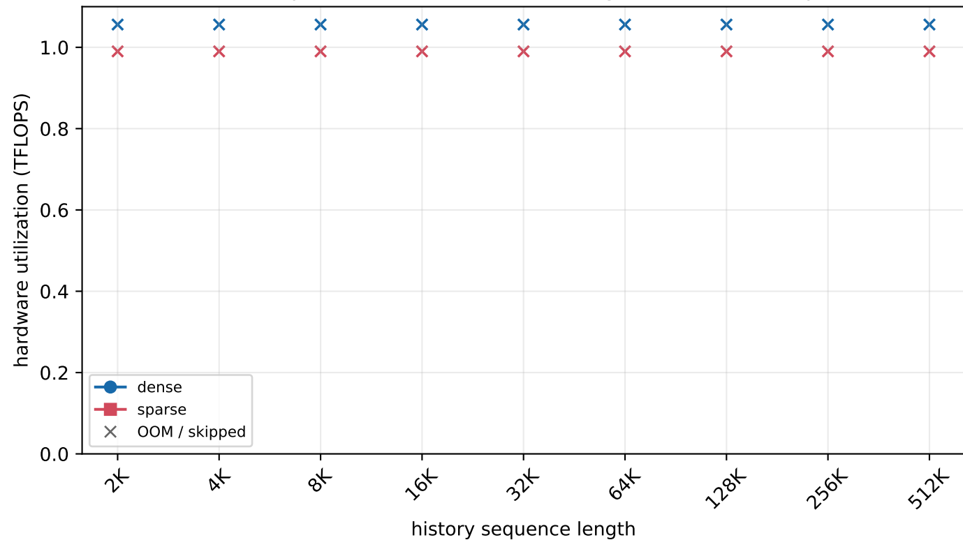
H800 MLA prefill - batch=256, new length=8K (chunked prefill)
