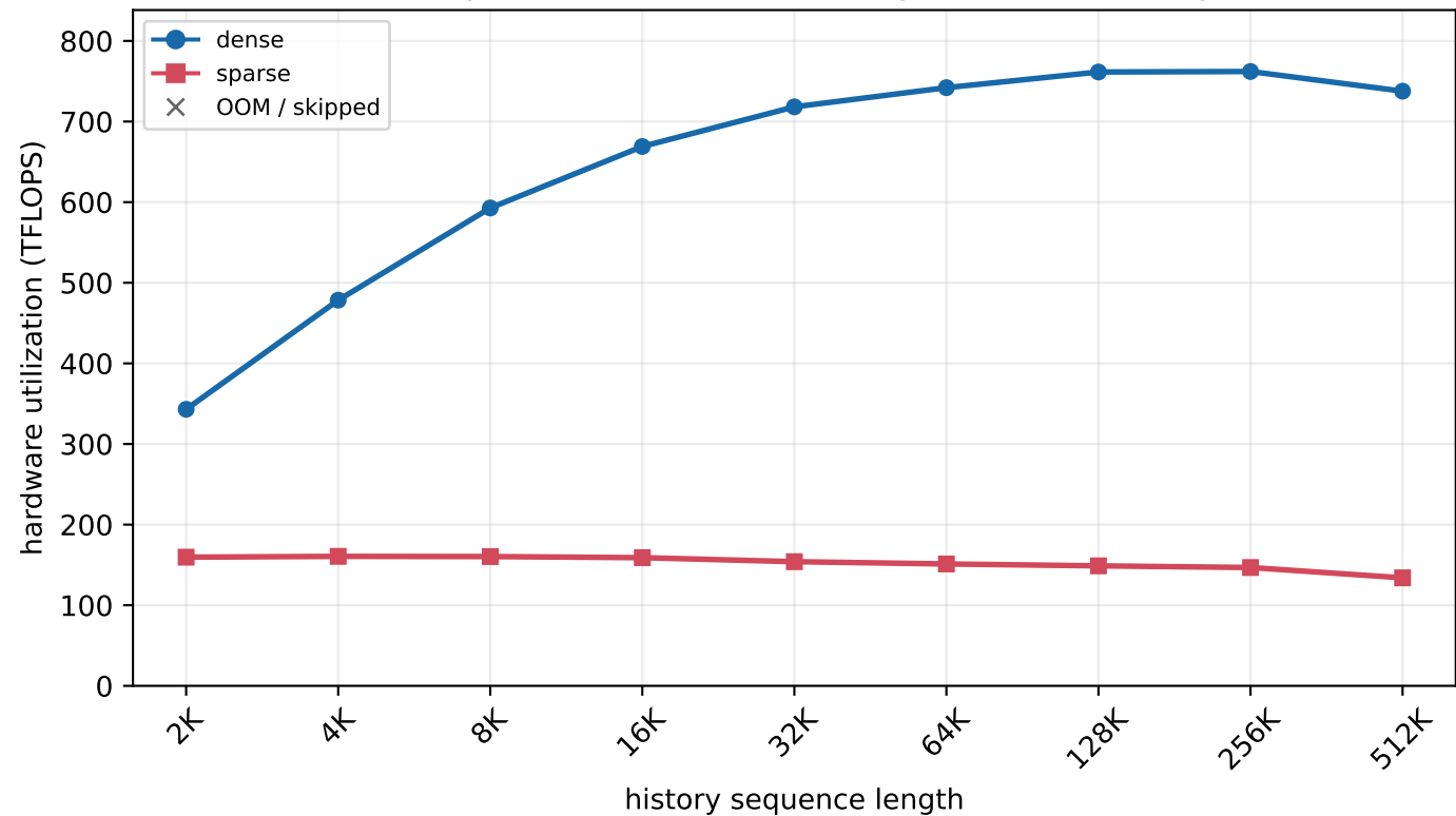
H800 MLA prefill - batch=2, new length=16 (chunked prefill)
