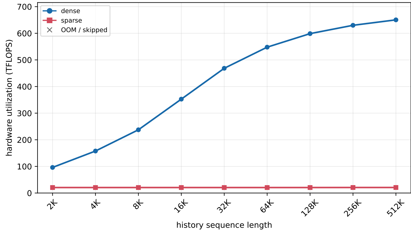
H800 MLA prefill - batch=2, new length=2 (chunked prefill)
