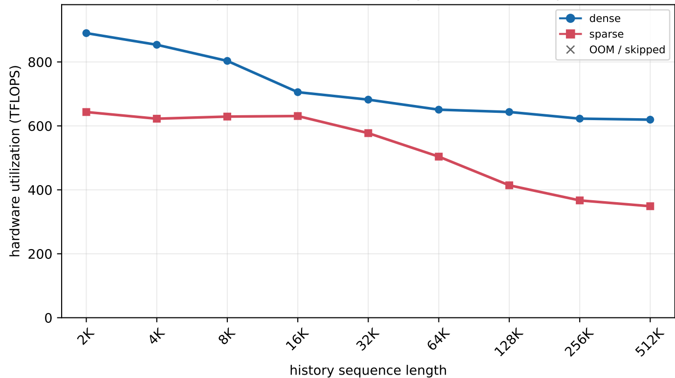
H800 MLA prefill - batch=2, new length=2K (chunked prefill)
