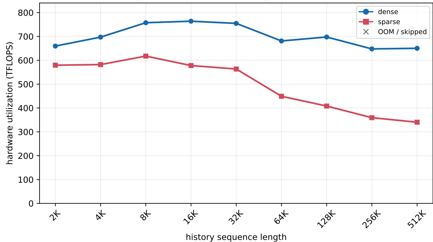
H800 MLA prefill - batch=2, new length=256 (chunked prefill)
