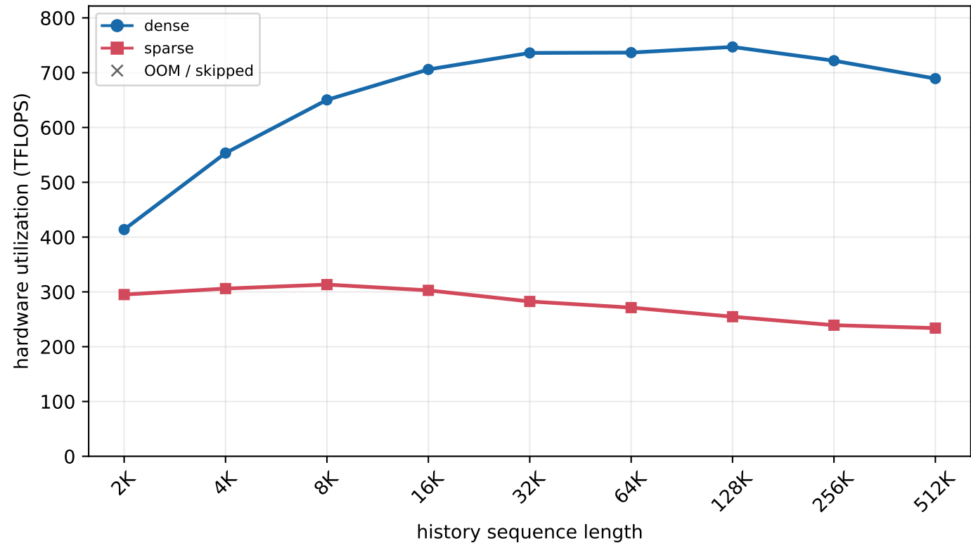
H800 MLA prefill - batch=2, new length=32 (chunked prefill)
