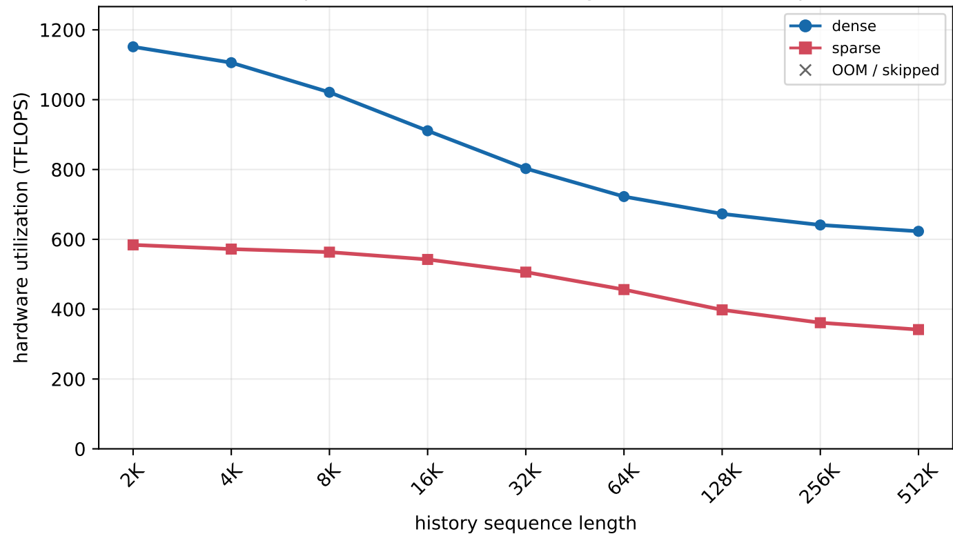
H800 MLA prefill - batch=2, new length=32K (chunked prefill)
