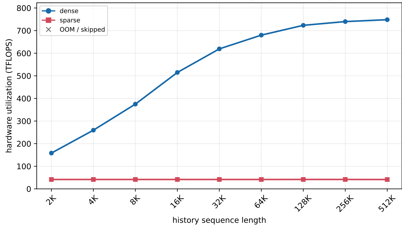
H800 MLA prefill - batch=2, new length=4 (chunked prefill)
