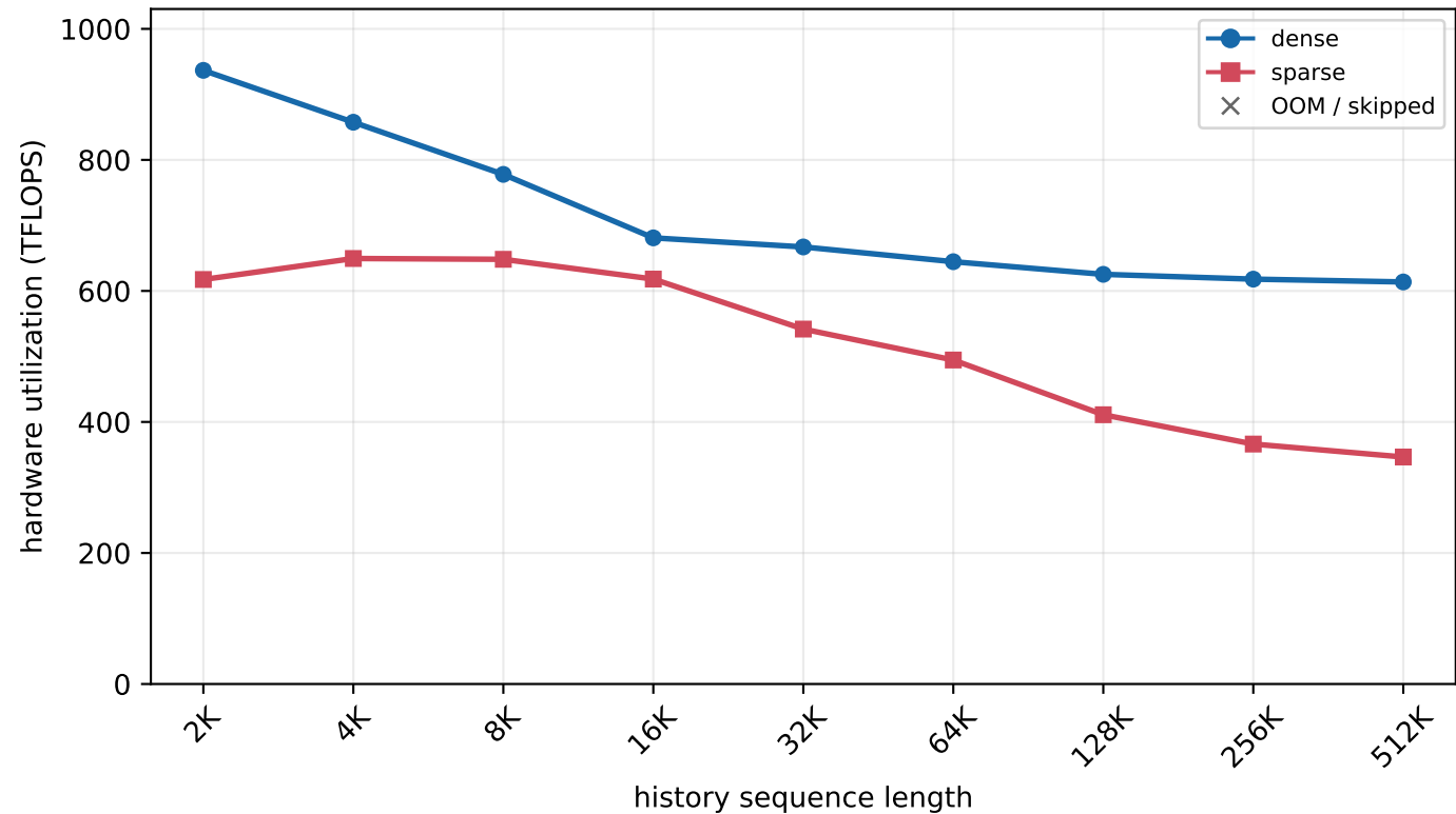
H800 MLA prefill - batch=2, new length=4K (chunked prefill)
