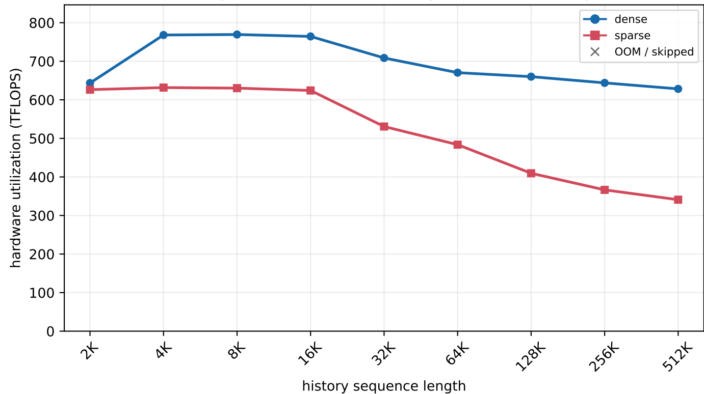
H800 MLA prefill - batch=2, new length=512 (chunked prefill)
