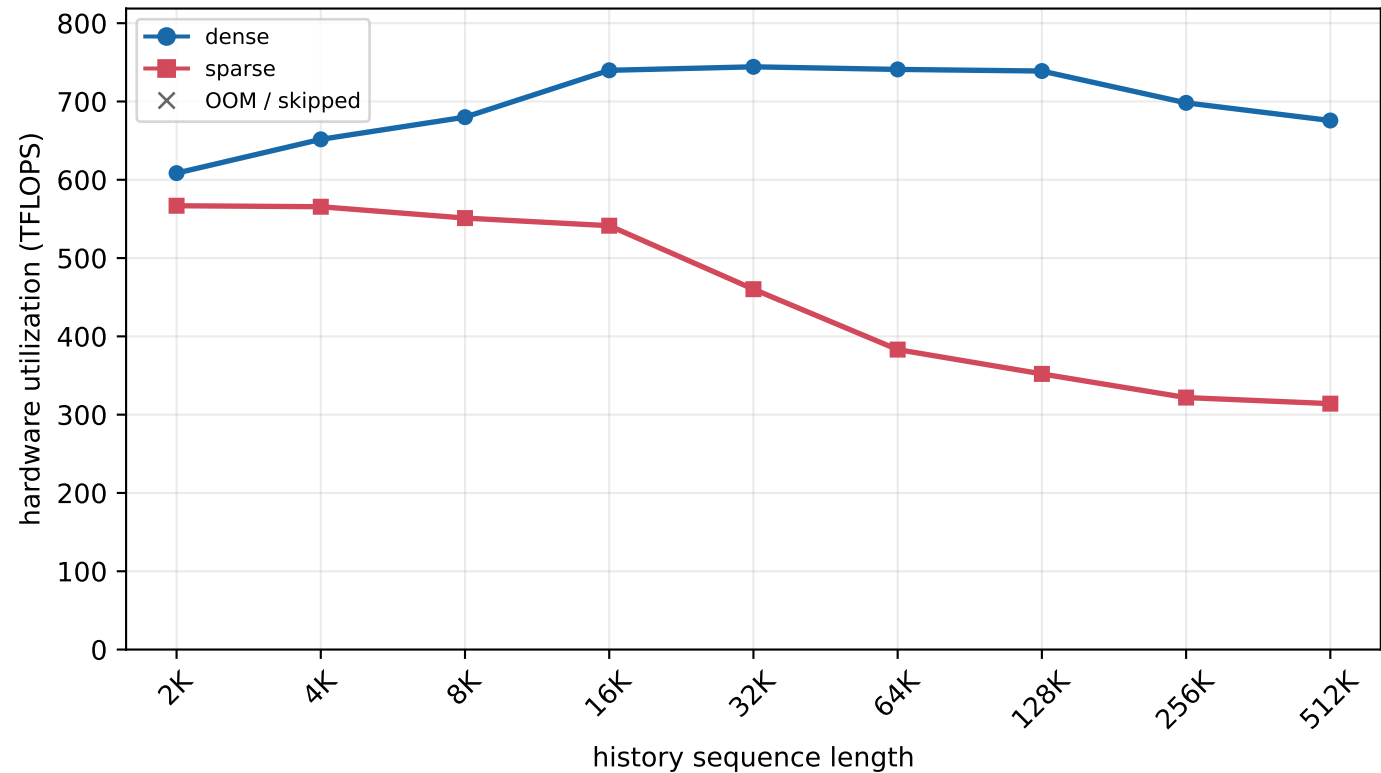
H800 MLA prefill - batch=2, new length=64 (chunked prefill)
