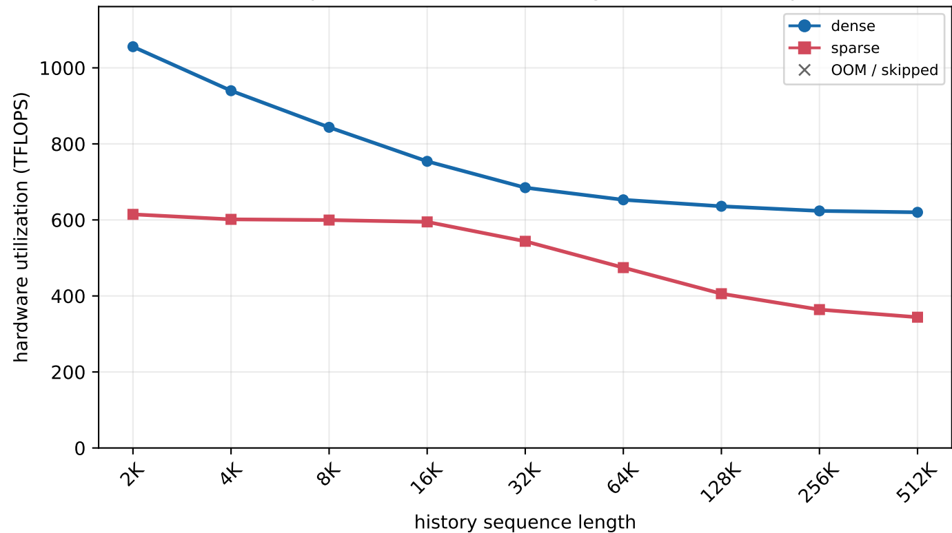
H800 MLA prefill - batch=2, new length=8K (chunked prefill)
