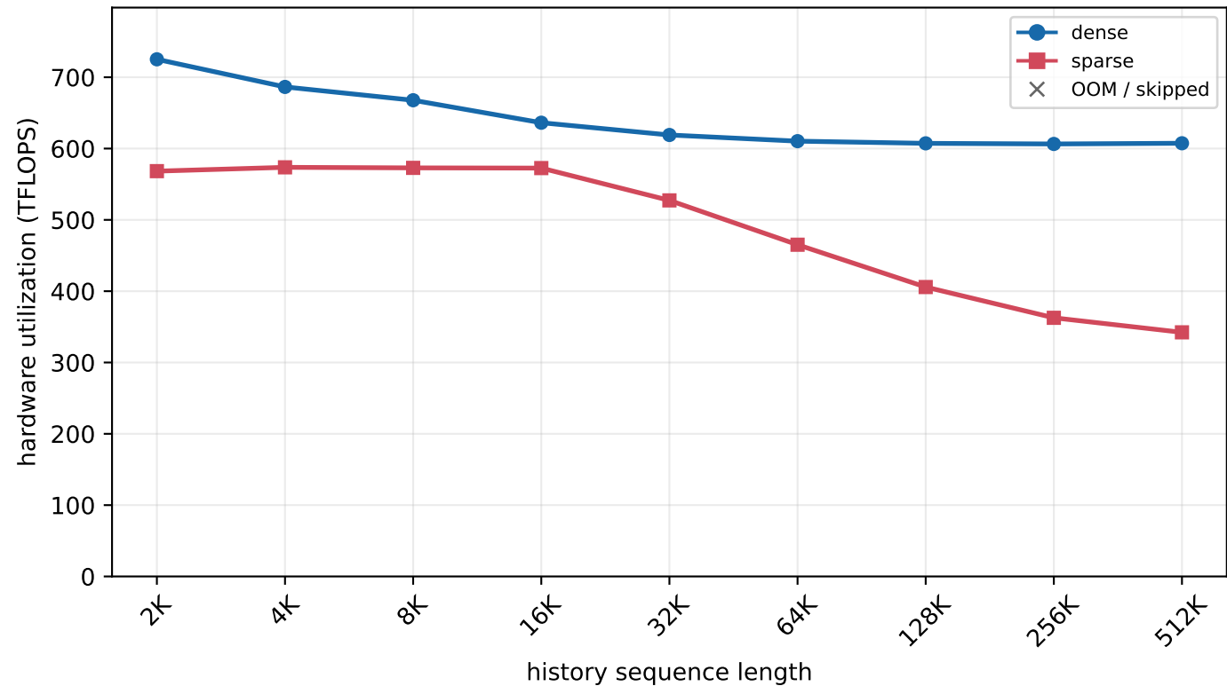
H800 MLA prefill - batch=32, new length=1K (chunked prefill)
