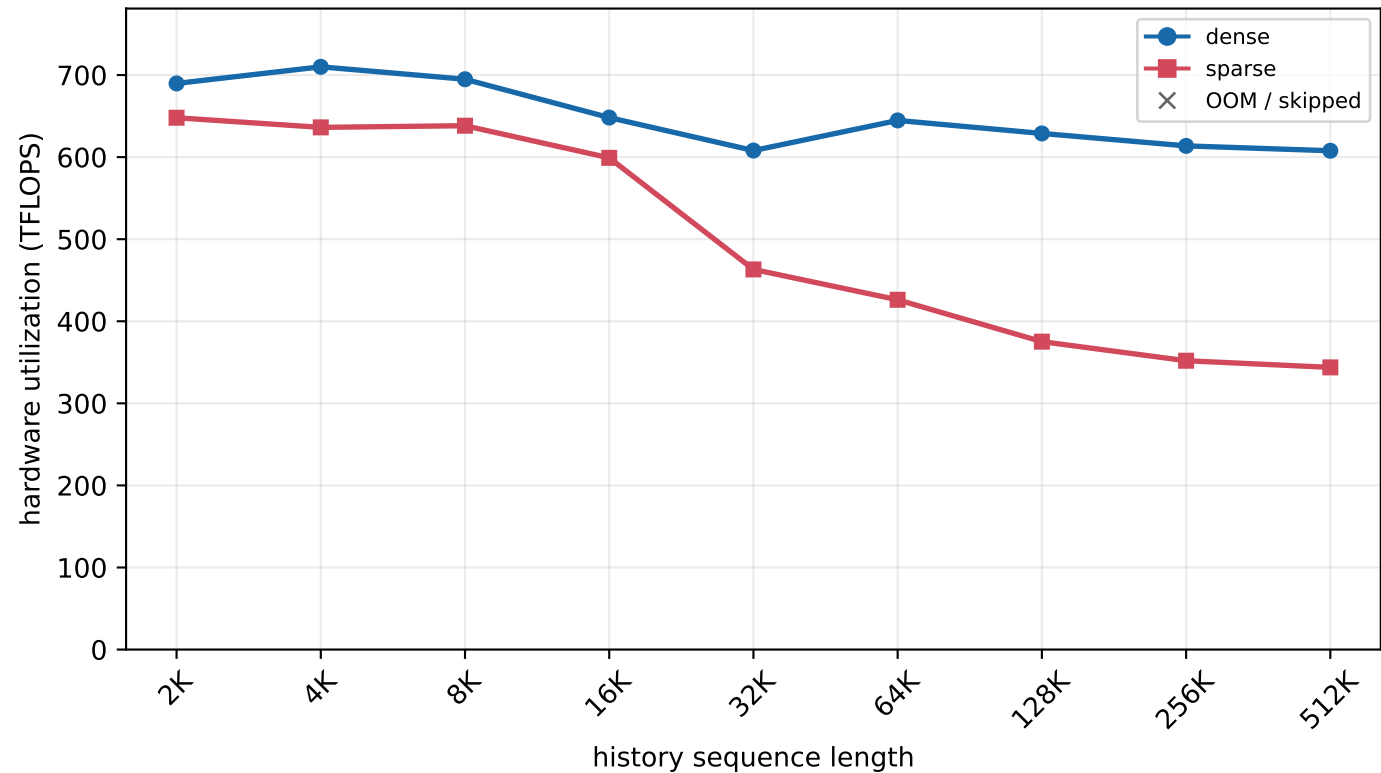
H800 MLA prefill - batch=32, new length=128 (chunked prefill)
