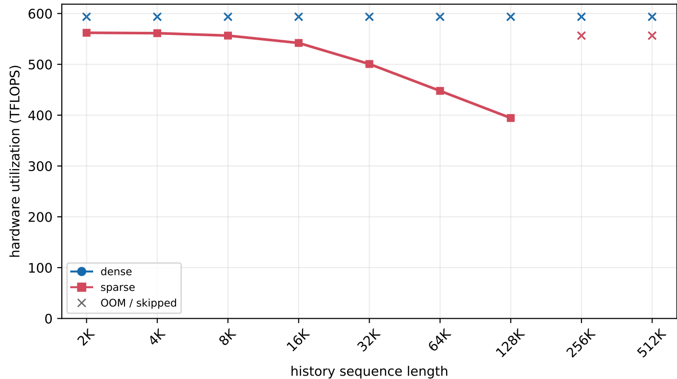
H800 MLA prefill - batch=32, new length=16K (chunked prefill)
